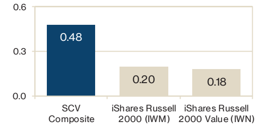
Sharpe Ratio (Trailing 5 YR) 1
