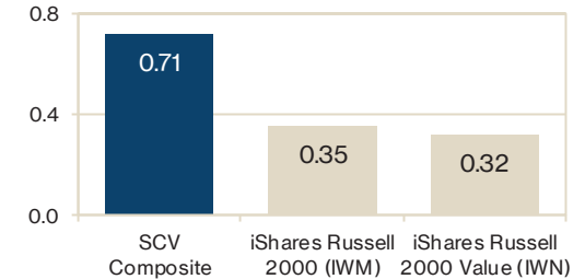
Sortino Ratio (Trailing 5 YR) 1 2
